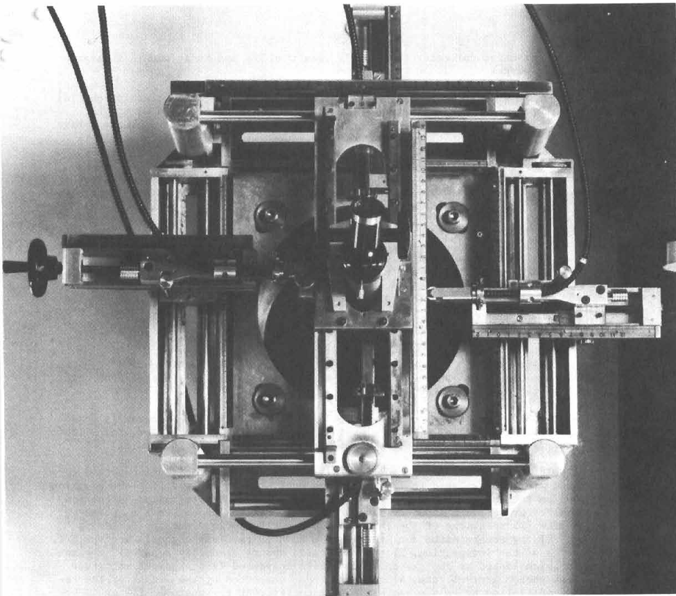
Fig. 2. The four XY-arm assembly for positioning the apertures in the focal plane.
