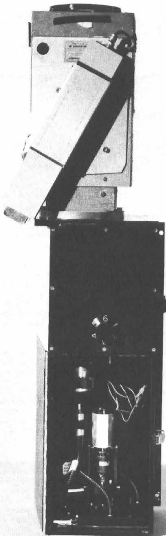
Fig. 3. The open Chopper Box showing the 4-into-1 fiber-optic adaptor, the motor which drives the chopper with its flexible drive, the P.F.R. cooler, and the P.A.R. preamplifier/discriminator.
